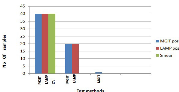
Figure 2. Comparative analysis of three procedures (Smear Microscopy, MGIT Culture and LAMP Test) employed in this study. X-axis represents the three test methods and Y-axis shows the number of samples. First three bars show that 40 out of total tested samples were simultaneously smear positive, MGIT culture positive and LAMP test positive. The second two bars represent those 20 samples which are Smear negative but positive for both MGIT culture and LAMP assay. Third one represents the sample which was negative on smear microscopy and LAMP test but positive for MGIT culture.
