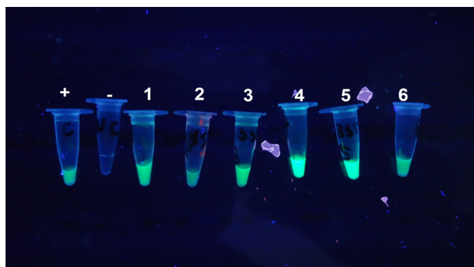
Figure 1. Visualization of LAMP amplicons under ultraviolet light with positive and negative control on the left and the test samples on the right.
