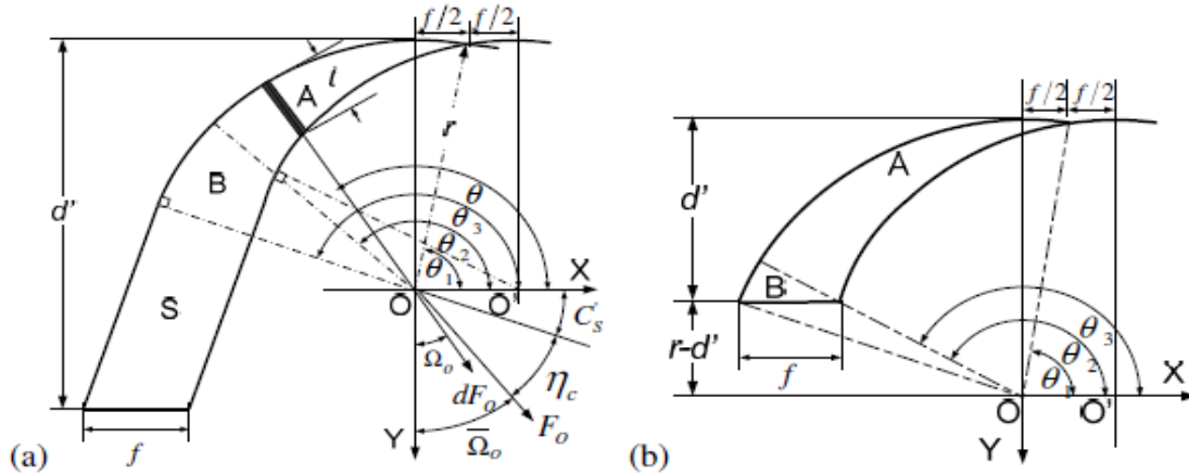
Fig. 5. Geometrical conditions of chip flow for a nose radius insert, (a) case 1: engaged side and nose radius edges and (b) case 2: engaged nose radius edge.
