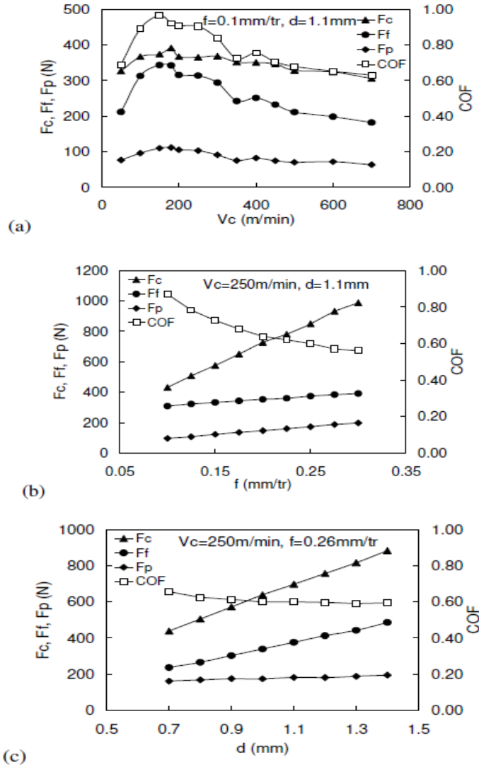
Fig. 6. Measured average cutting force components and apparent coefficient of friction in the case of turning with flatted insert.
