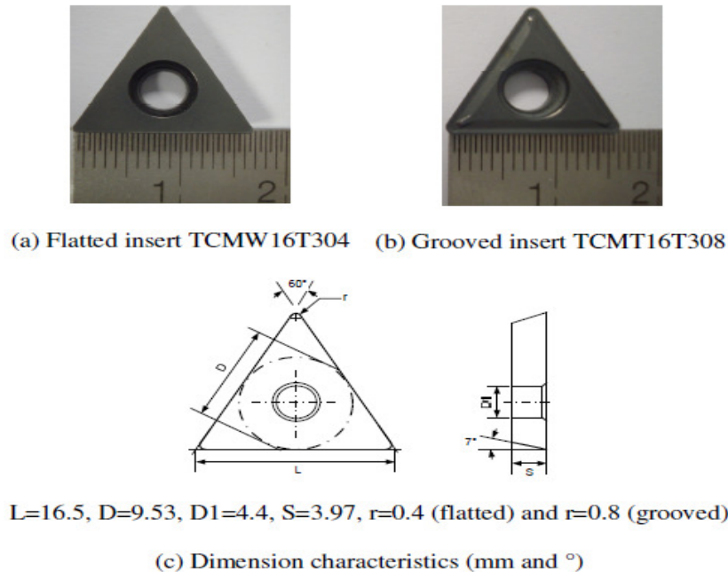
Fig. 2. Flatted and groove inserts used in turning tests.
