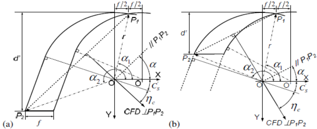
Fig. 4. Geometric conditions of chip flow for a nose radius insert, based on geometrical Colwell model.
