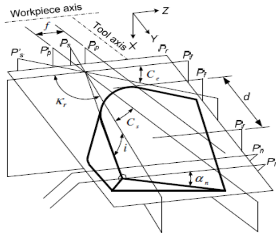
Fig. 3. Definition of the main cutting angles for nose radius insert.
