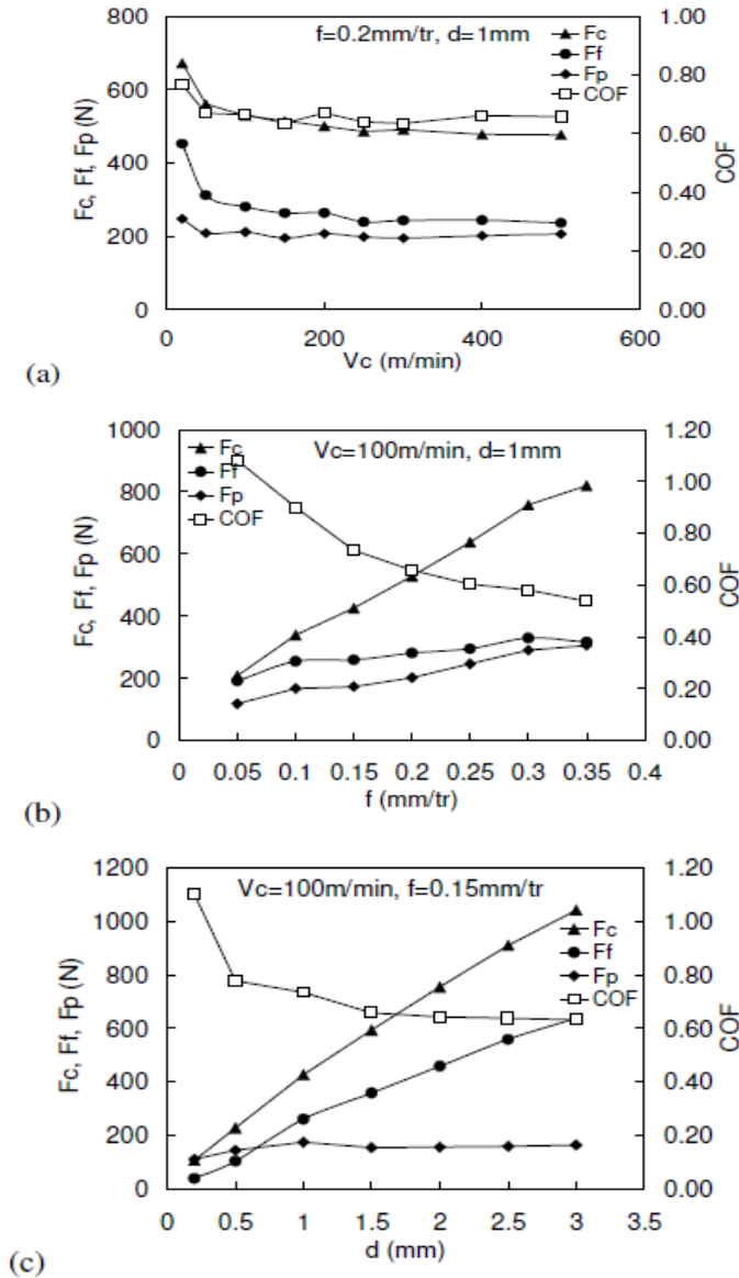
Fig. 7. Measured average cutting force components and apparent coefficient of friction in the case of turning with grooved insert.
