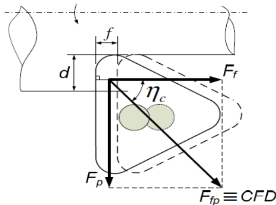
Fig. 3. Definition of CFD from feed and depth of cut force components ( \alpha_n = i = 0 ).
