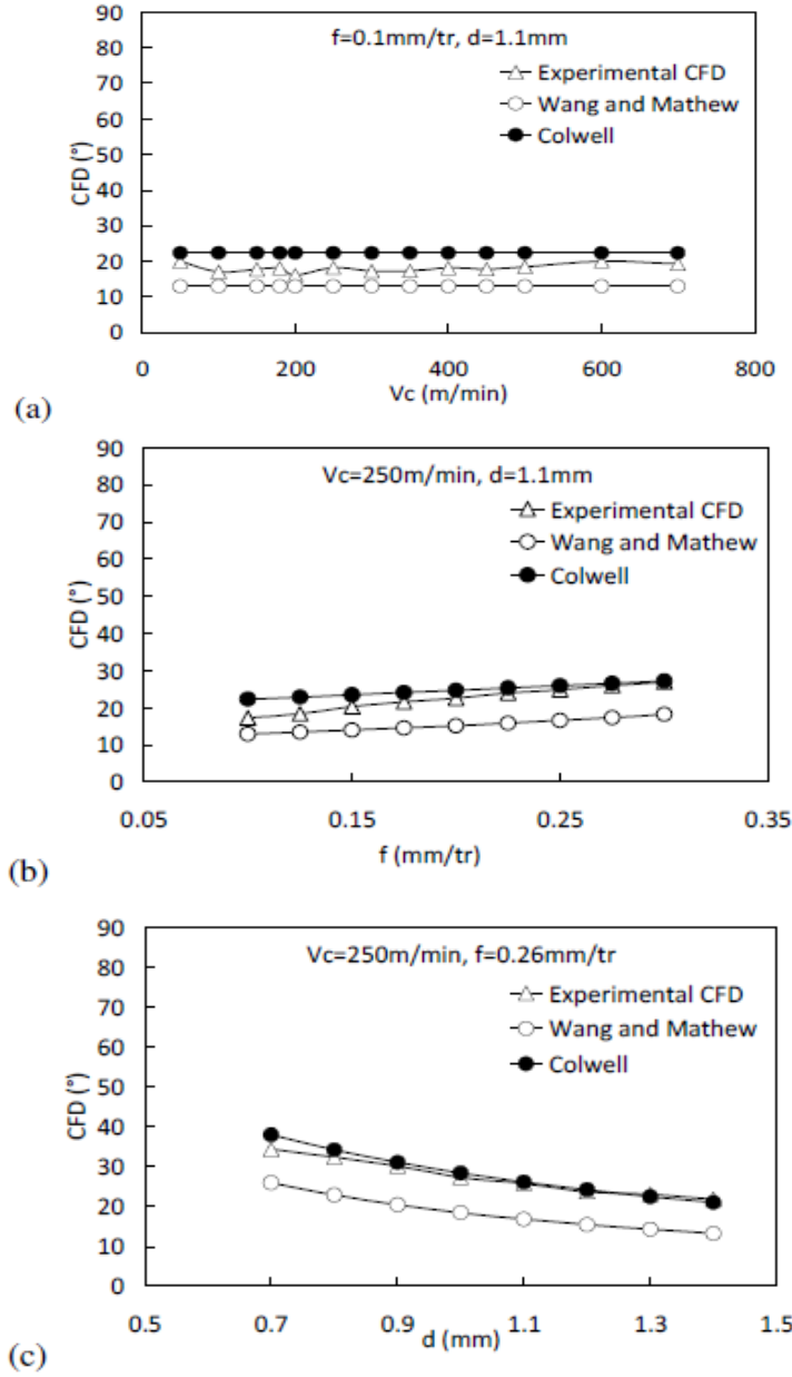
Fig. 8. Comparison between predicted and experimental CFD in the case of turning with flatted uncoated inserts.
