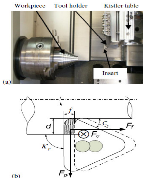
Fig. 1. (a) Experimental setup and (b) definition of measured cutting force components and cutting configuration ( C_s = 0^\circ or \kappa_r = 90^\circ , C_e = 30^\circ , i = 0^\circ , \alpha_n = 0^\circ ).
