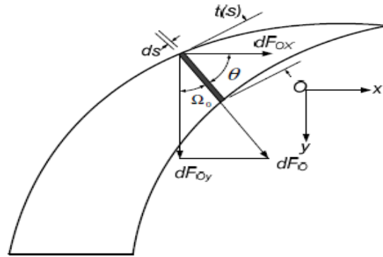
Fig. 6. Model for predicting chip flow angle caused by nose radius cutting edge.
