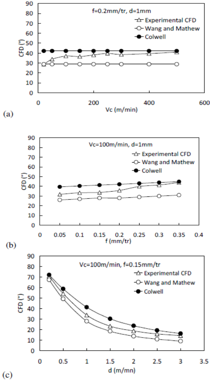
Fig. 9. Comparison between predicted and experimental CFD in the case of turning with grooved coated inserts.
