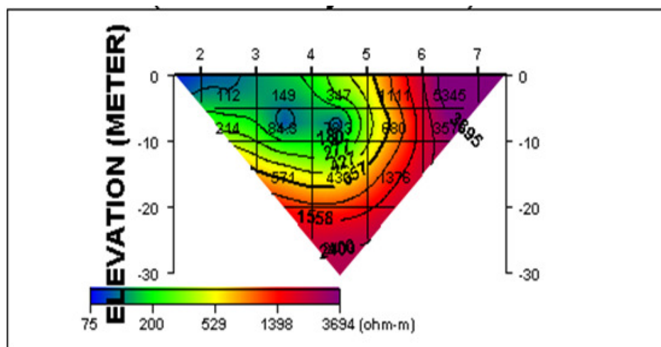
Figure 4 Resistivity Structure along Profile 1
