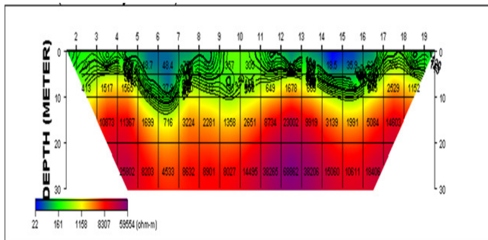
Figure 9 Resistivity Structure along Profile 6
