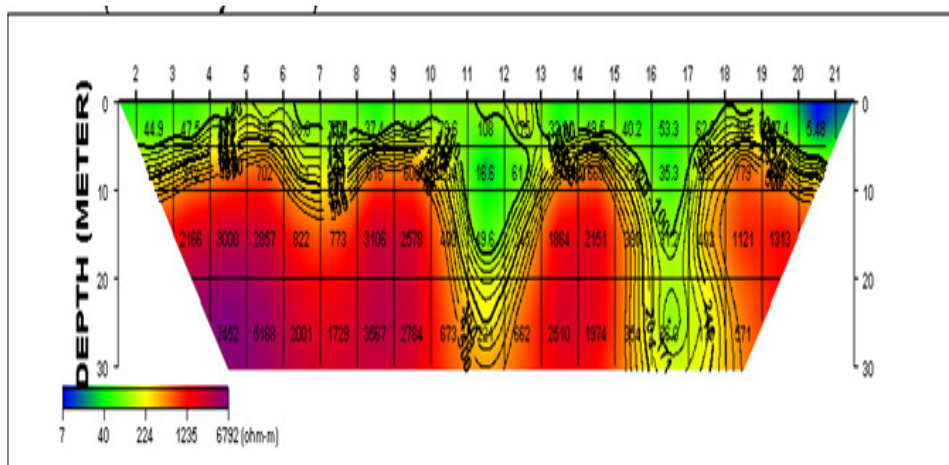
Figure 8 Resistivity Structure along Profile 5
