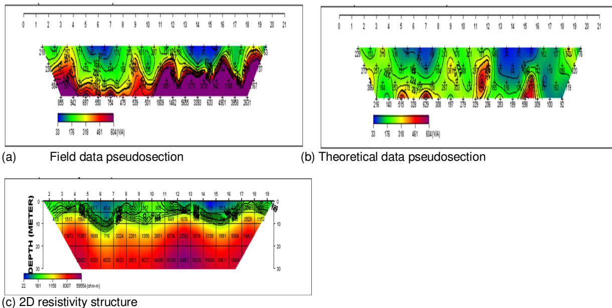
Figure 3 Resistivity Images of Profile 6
