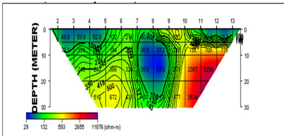
Figure 7 Resistivity Structure along Profile 4
