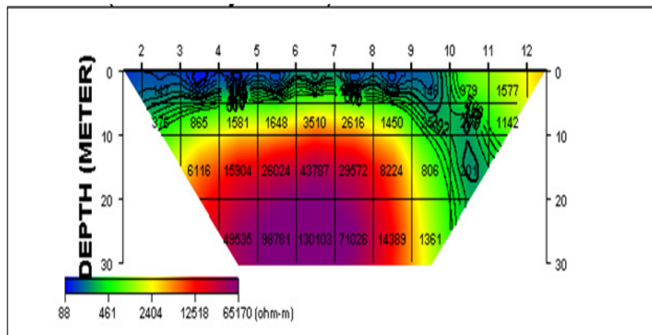
Figure 5 Resistivity Structure along Profile 2
