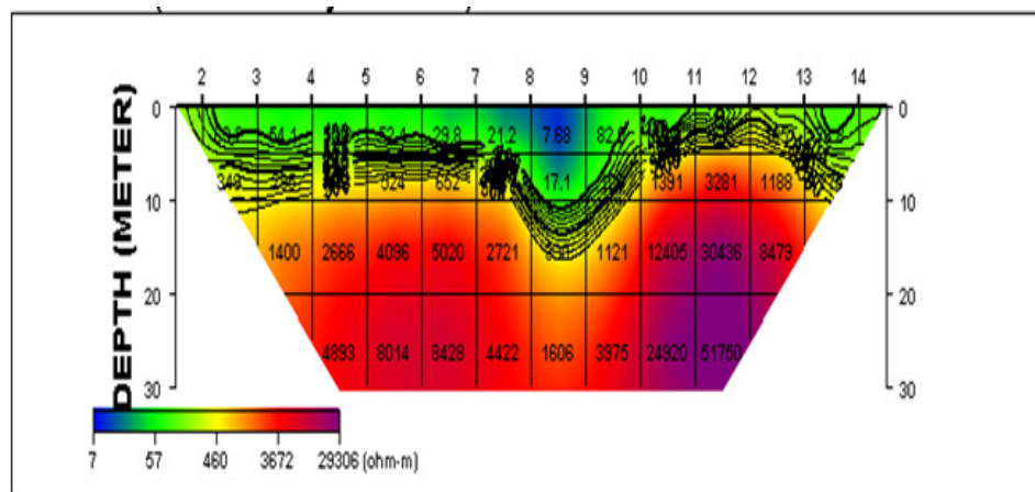
Figure 6 Resistivity Structure along Profile 3
