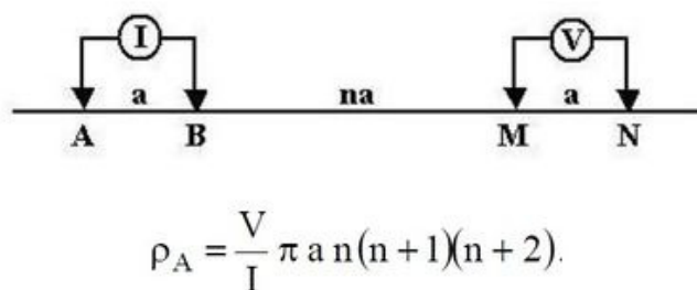
Figure 2 Dipole-Dipole configuration and apparent resistivity
